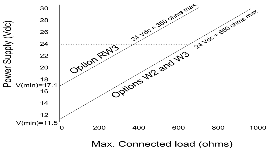
Figure 2 Loop Impedance versus Power Supply Voltage
