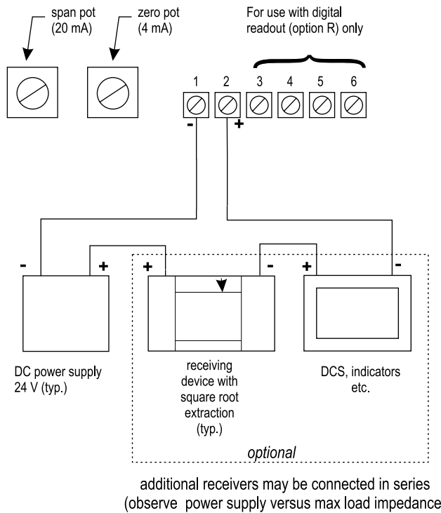
Figure 1 Connection Diagram
